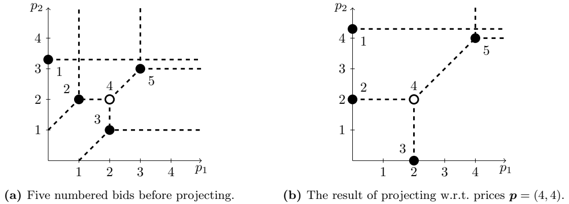
Figure 6: Example of the project operation w.r.t. prices \mathbf{p} = (4, 4) on five bids numbered from 1 to 5 shown in (a). The projected bids are shown in (b). Note that only the negative bid is unchanged, as it demands all goods, including the reject good.
