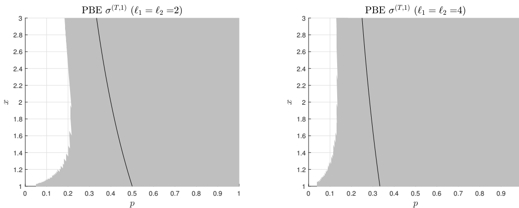
Figure 5: Illustration of Proposition 6 for different values of (p, x) . The shaded region depicts the pairs of (p, x) such that \sigma^{(T,1)} is a PBE for sufficiently high discount factors for some T in the synchronous model without a public randomization device. Left: \ell_1 = \ell_2 = 2 . Right: \ell_1 = \ell_2 = 4 . In both panels, the solid curve illustrates the threshold below which \sigma^G is a unique PBE for sufficiently high discount factors in our main model with asynchronous moves. By Proposition 5, the shaded area would occupy the entire region (except at p = 0 ) when x \leq 1 .
