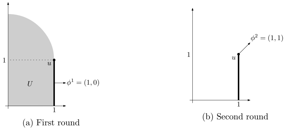
Figure 4: Rationalizing a Pareto optimal point in two rounds of sequential utilitarian welfare maximization.
