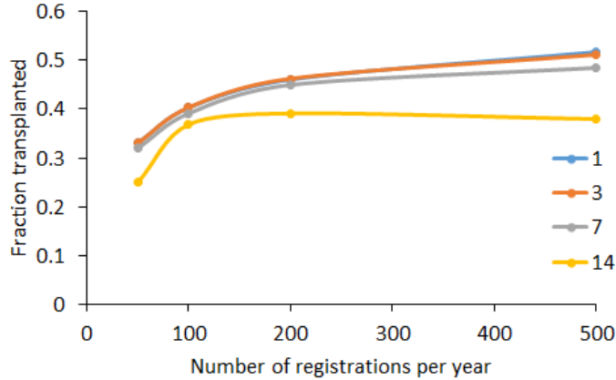
Figure 6: Batching policies for different arrival rates using NKR data (from Agarwal et al. (2018)). Each plot corresponds to the batch size in days.
